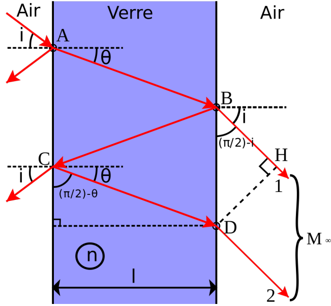
FIGURE 6 – Fabry-Perot
